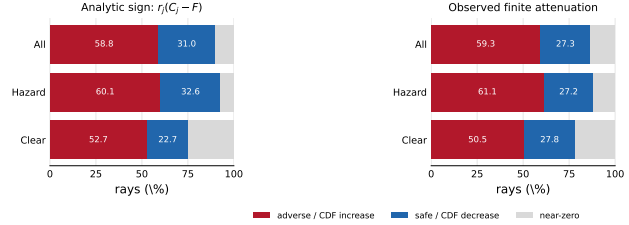
Figure 4. M49 attenuation sign boundary on 99,208 frozen rays. Red denotes the analytically adverse direction (left) or an observed increase in the pre-boundary CDF (right); blue denotes the corresponding safe/decreasing direction. The result is descriptive and is never converted into a selection rule.
