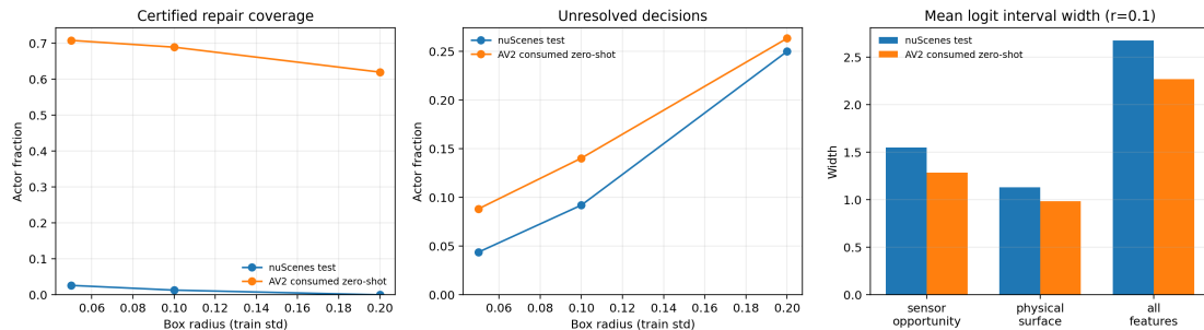
Figure 3. Frozen P7-C interval audit. Left/center: robust-select coverage and unresolved fraction across pre-registered radii. Right: sensor-opportunity boxes induce wider logit intervals than physical-surface boxes. The high AV2 certified coverage does not erase the 47 stable false repairs.
