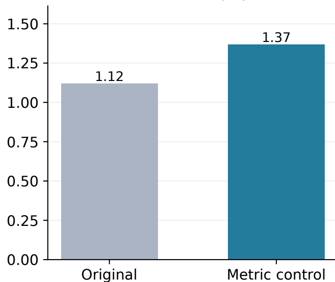
C2: MISS (%)
