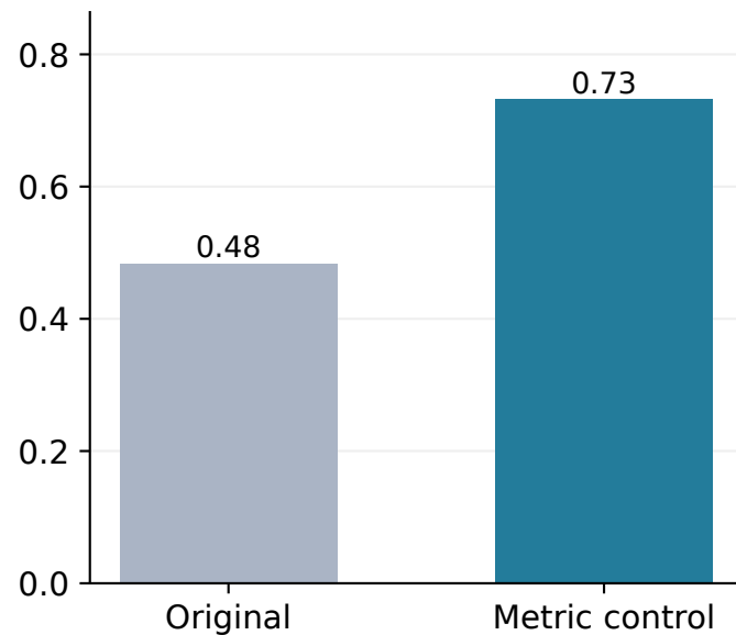
C2: MISS (%)
