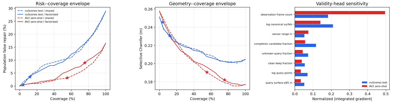
Figure 2. Frozen P7 safety envelope. Left and center: risk-coverage and geometry-coverage curves; stars mark the unchanged nuScenes-calibrated thresholds and never select an AV2 operating point. Right: Integrated Gradients relative to the nuScenes-training mean [17]. AV2 reliance on observation-frame count exposes a sensor-opportunity shortcut. Curves and attributions are descriptive rather than a cross-domain certificate.
