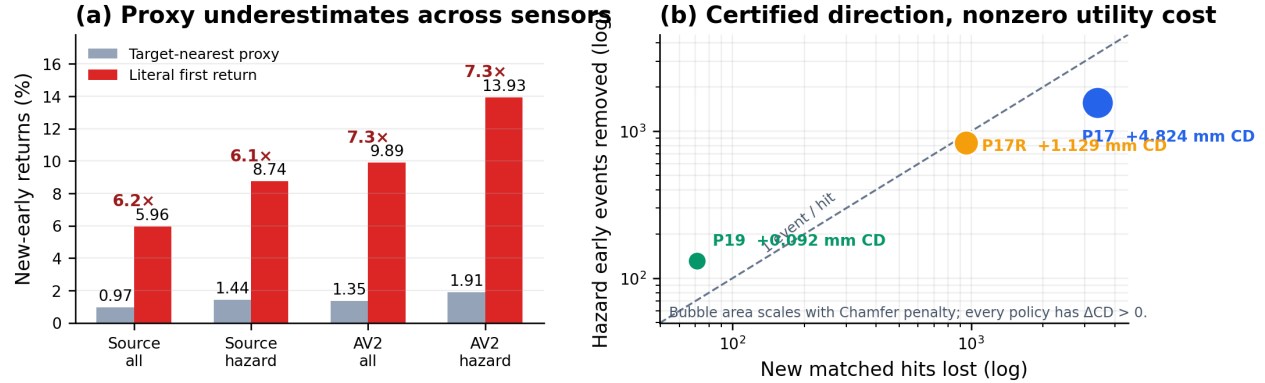
Figure 1. Frozen literal first-return boundary. (a) The target-nearest proxy understates total and hazardous-Actor new-early exposure on both source and AV2. (b) Deleting points is directionally safe for early returns, but every frozen source policy loses matched hits and worsens Chamfer. Bubble area scales with the Chamfer penalty. Ratios are consumed-source or consumed-AV2 diagnostics, not fresh transfer or road-safety bounds.
