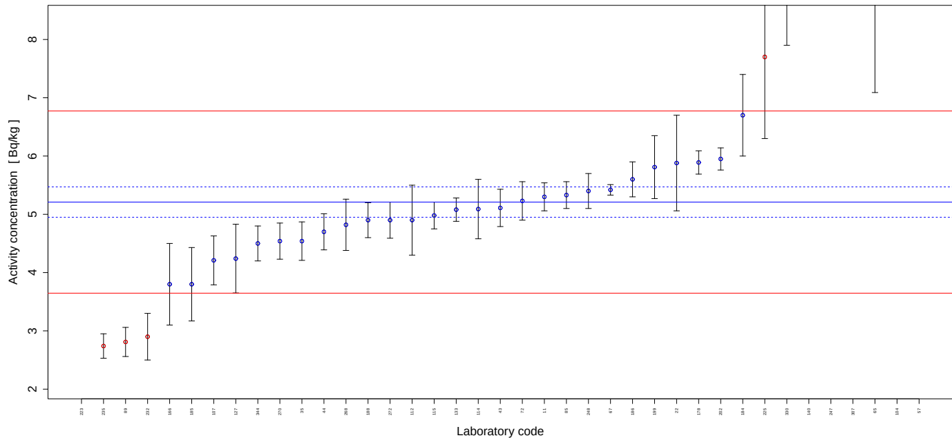
FIGURE 22. Reported results and evaluation parameters for Po-210. Blue points represent accepted scores, whereas yellow and red represent warning and not accepted scores respectively.
