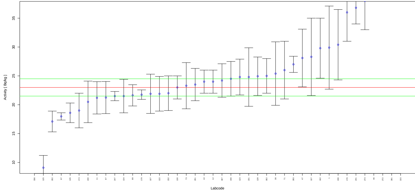
FIGURE 67. Reported results and evaluation parameters for U-238 in Sample 4.
