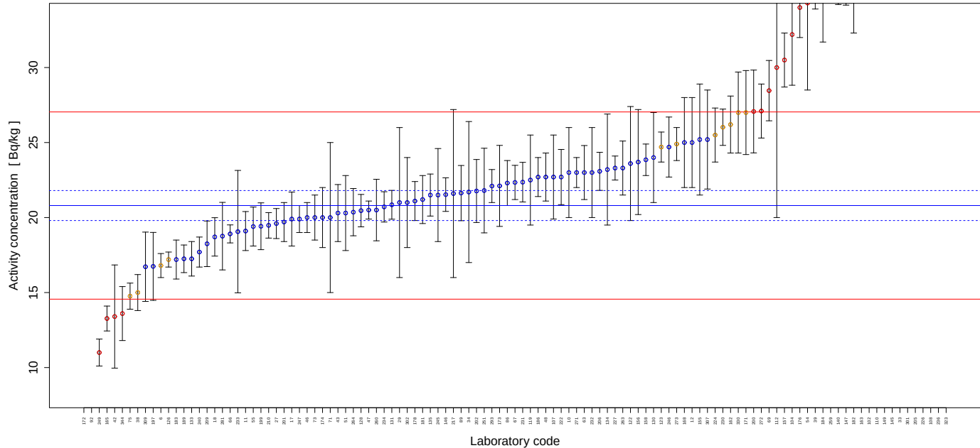
FIGURE 46. Reported results and evaluation parameters for Ra-226. Blue points represent accepted scores, whereas yellow and red represent warning and not accepted scores respectively.
