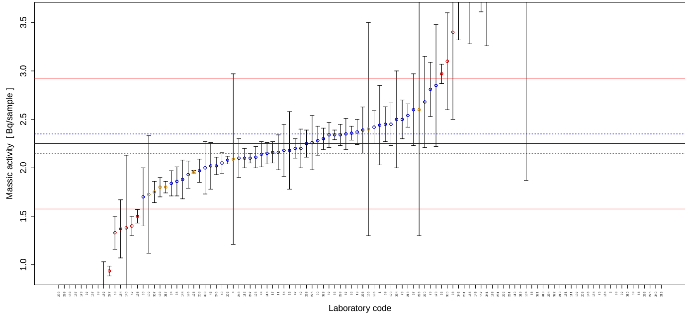
FIGURE 56. Reported results and evaluation parameters for Sr-90. Blue points represent accepted scores, whereas yellow and red represent warning and not accepted scores respectively.
