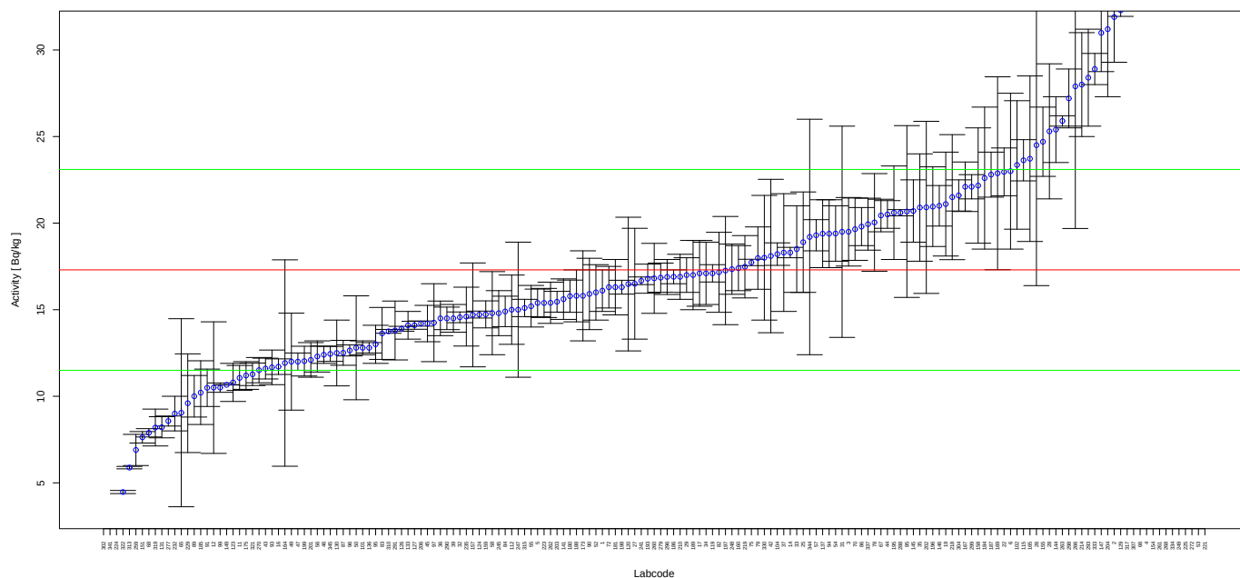
FIGURE 62. Reported results and evaluation parameters for gross beta in Sample 1.
