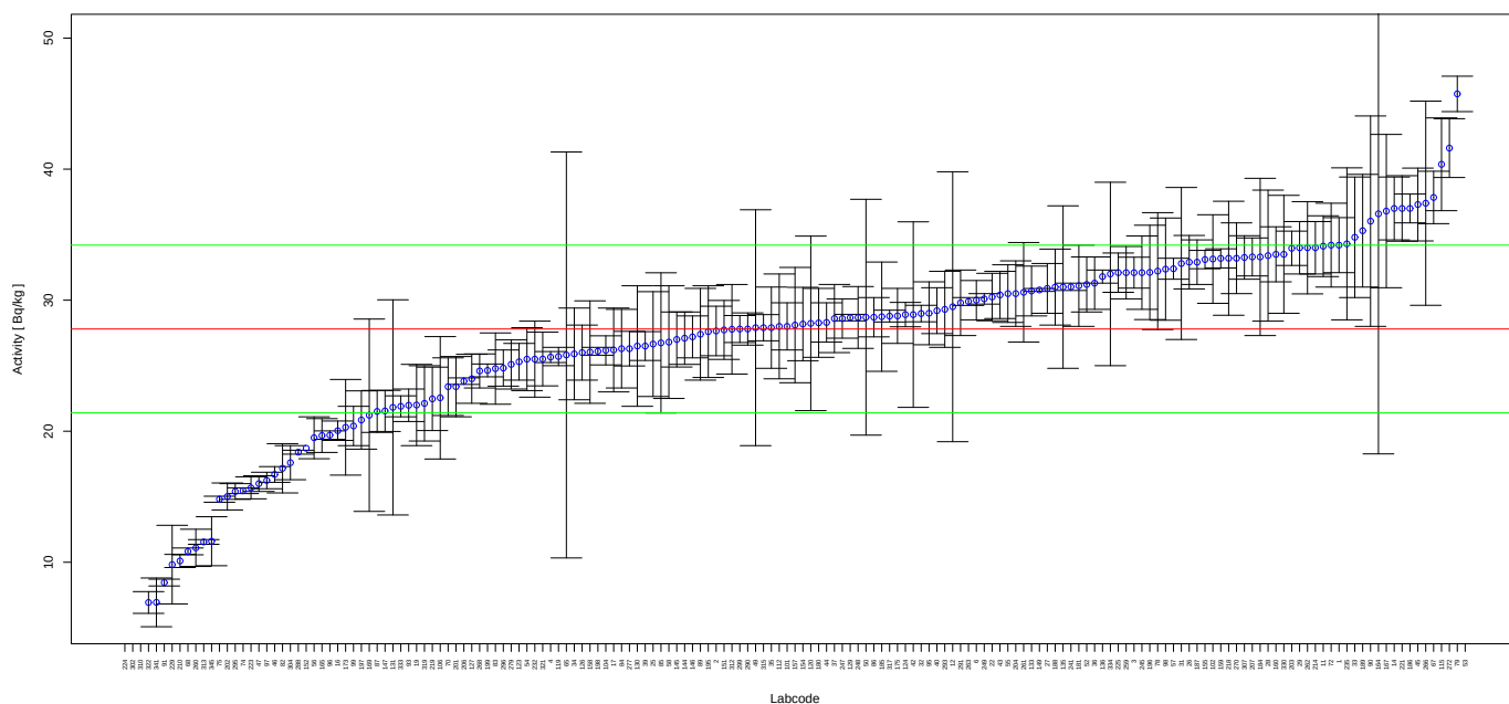
FIGURE 61. Reported results and evaluation parameters for gross alpha in Sample 1.
