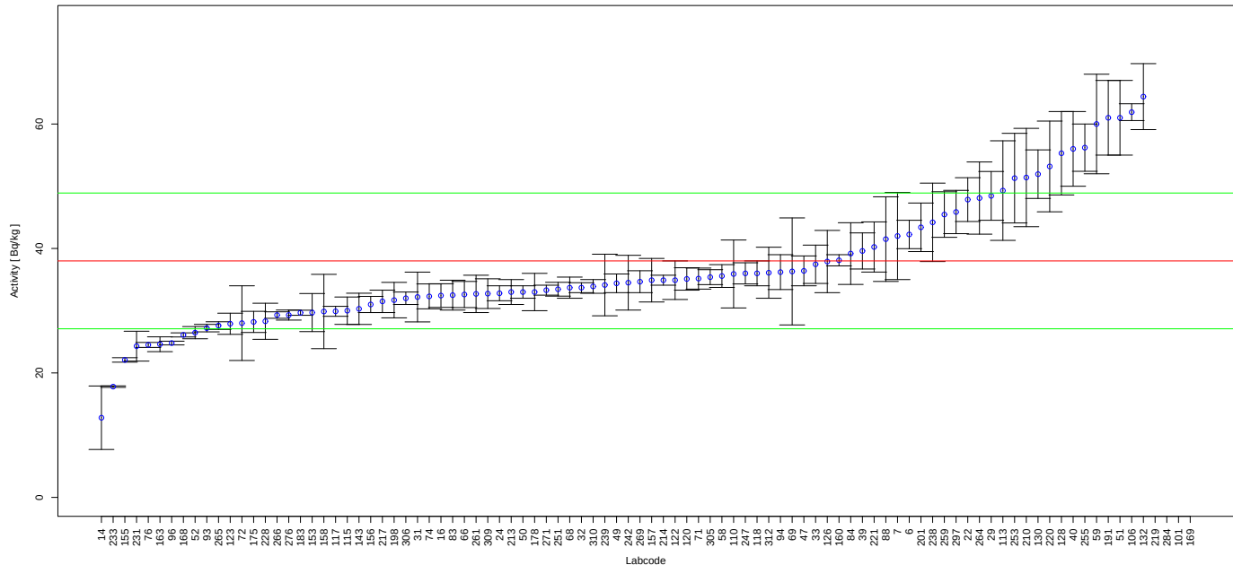
FIGURE 59. Reported results and evaluation parameters for Ra-226 in Sample 7.
