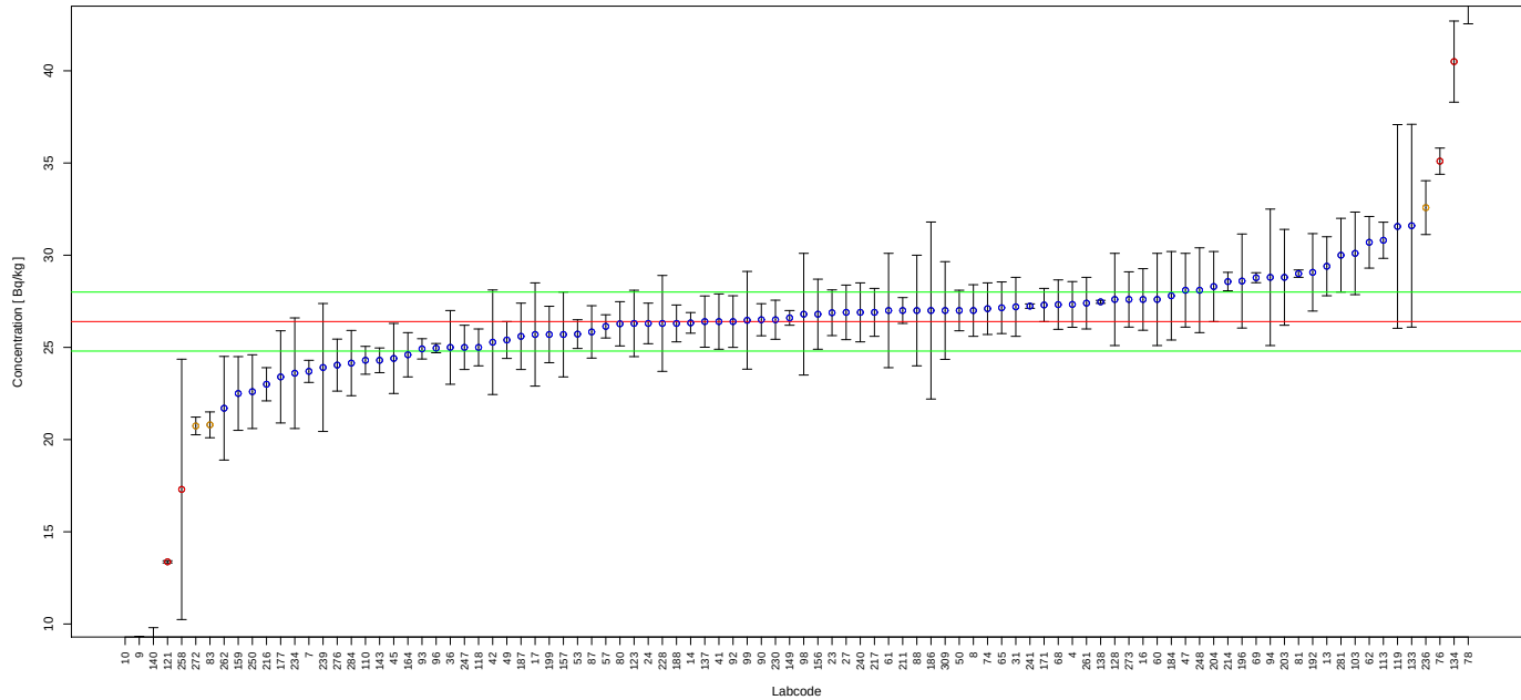
FIGURE 4. Reported results and evaluation parameters for Sr-90. Blue points represent accepted scores, whereas yellow and red represent warning and not accepted scores respectively.
