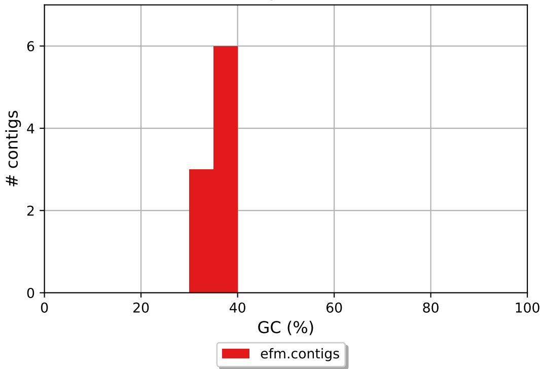
efm.contigs GC content
