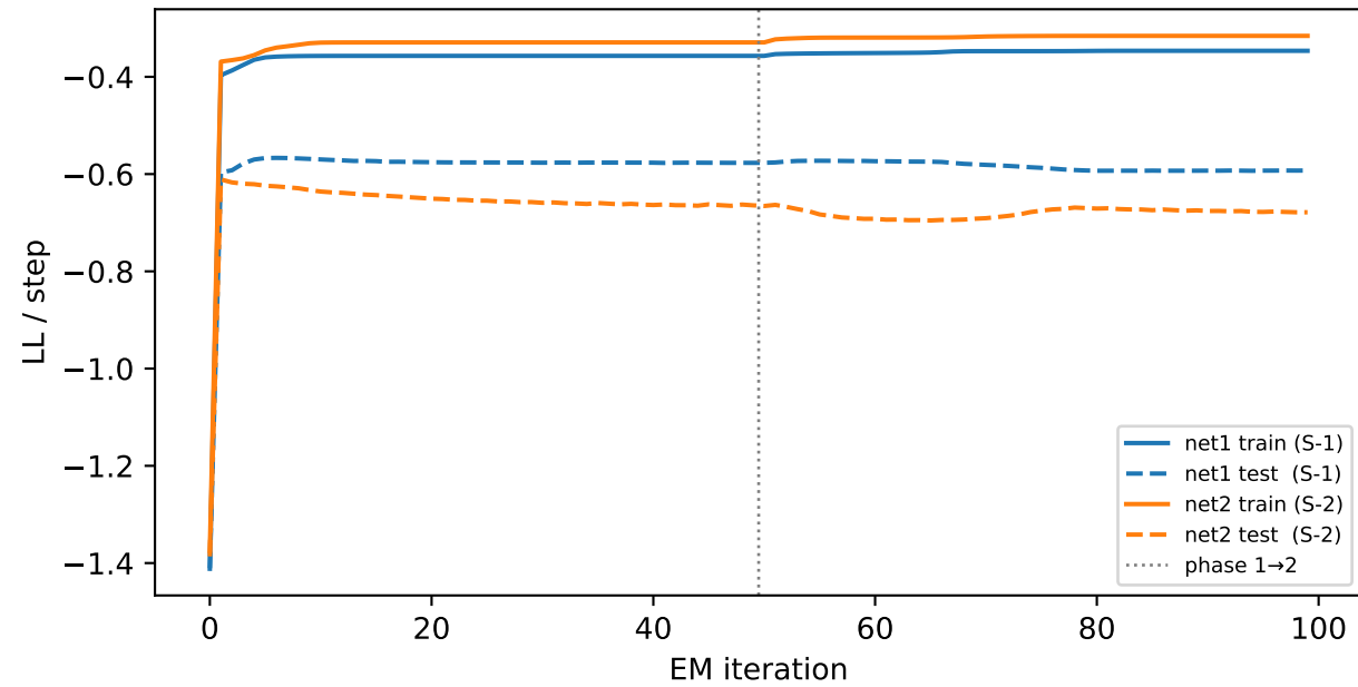
compressed K=2, seed=30 (full)
