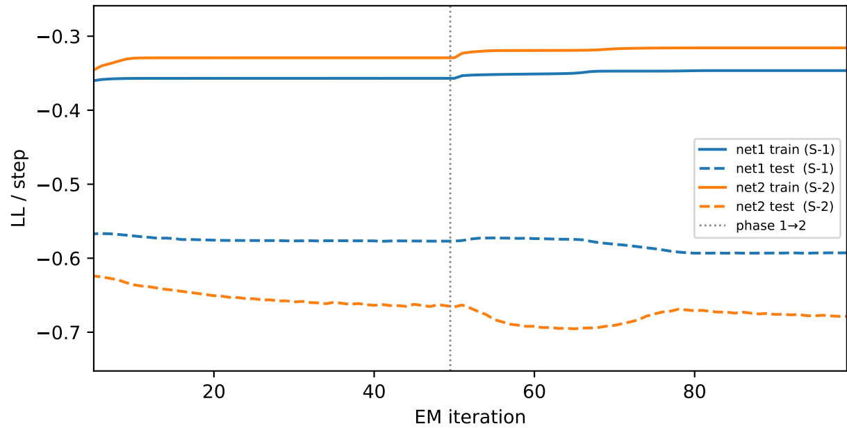
compressed K=2, seed=30 (iter 5+)
