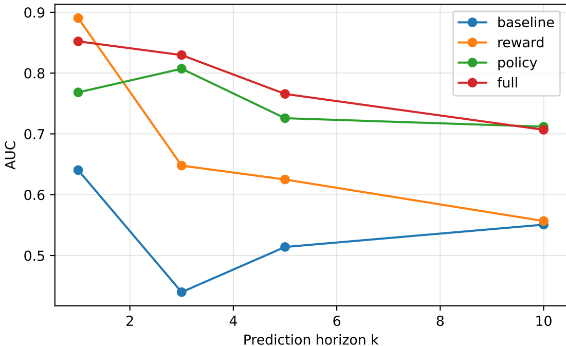
Escalation potential: AUC (compressed, net1)
