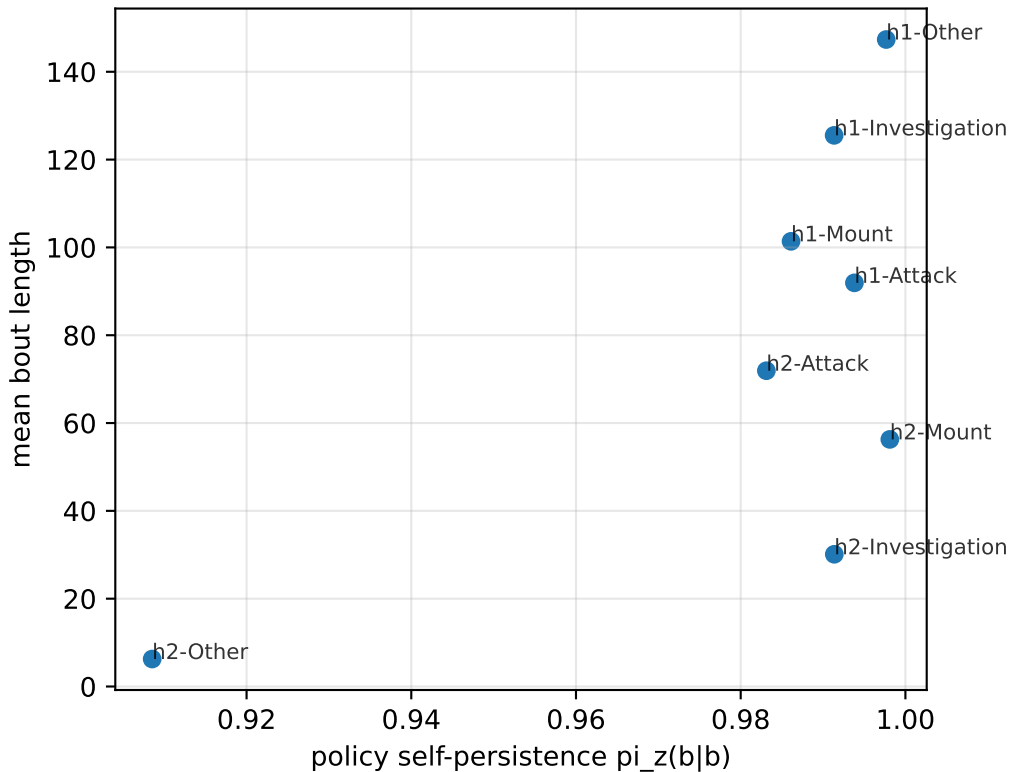
Policy self-persistence vs mean bout length (standard, net2)
