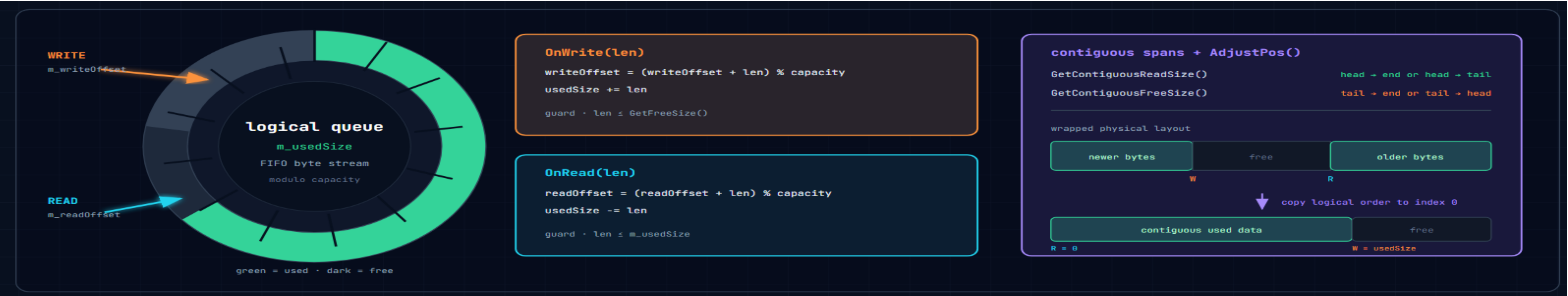
1) RIORingBuffer.h
