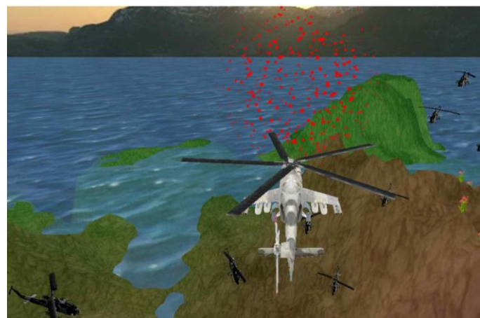
Sparkle
