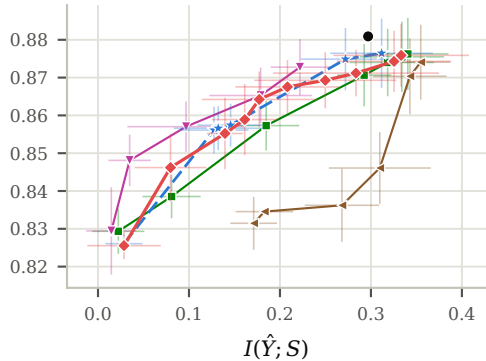
Continuous S
