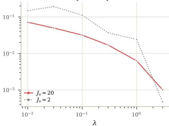
empirical supIPM (test split)
