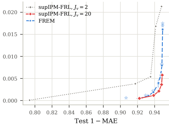
worst-case L_\infty -GDP
