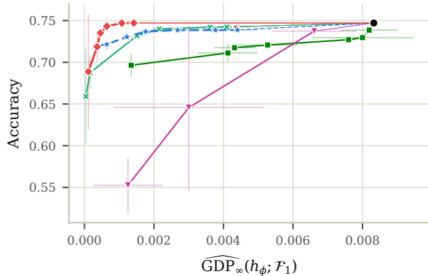
Pokec-z
