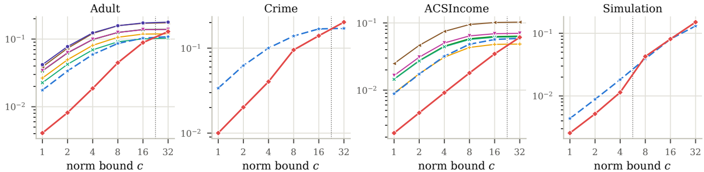
worst-case L_\infty -GDP
