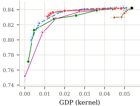
Continuous S
