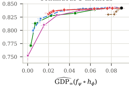
Continuous-S methods
