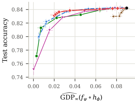
Continuous- S methods
