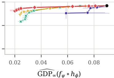
Binary-S methods
