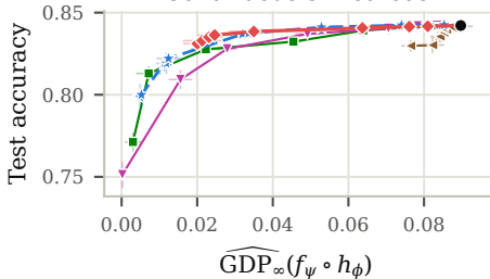
Continuous-S methods
