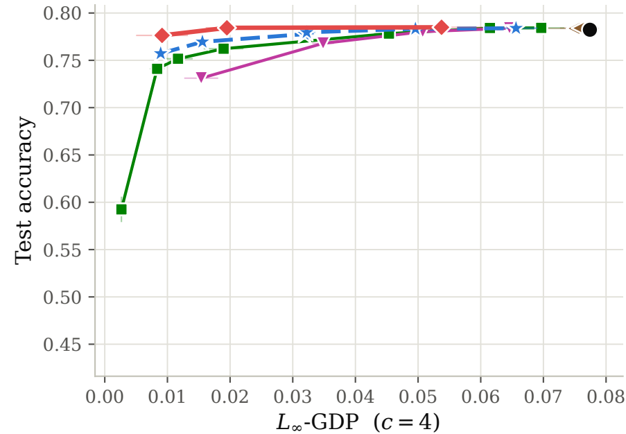
Continuous S
