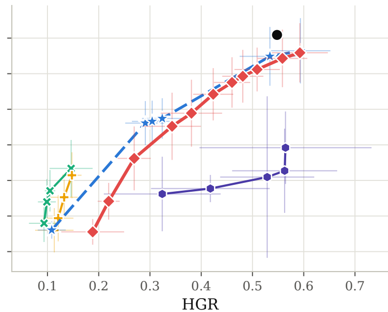
Binary S (mean)
