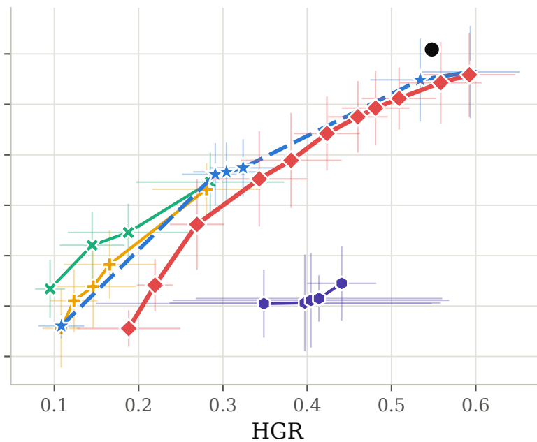
Binary S (median)
