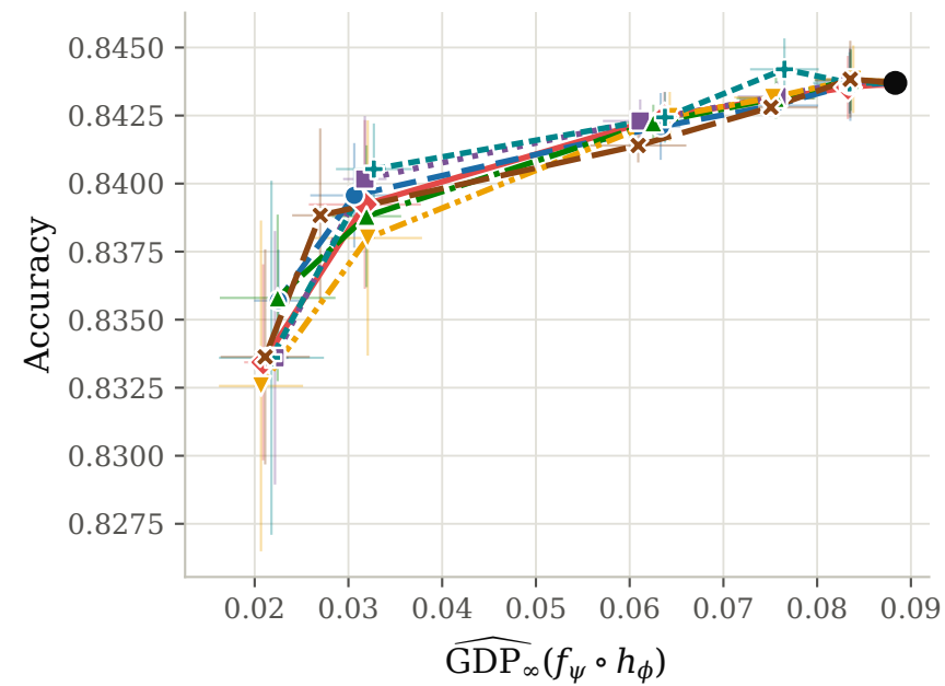
Adult
