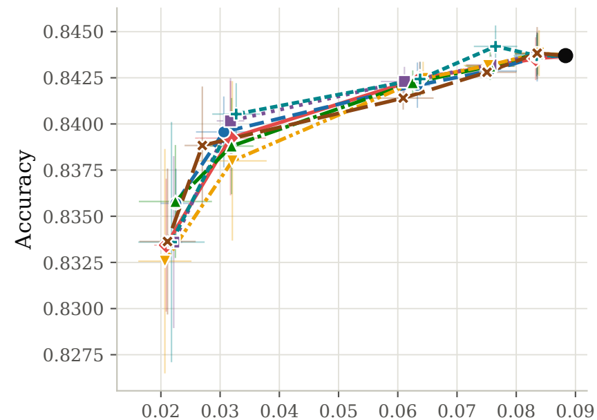
Adult
