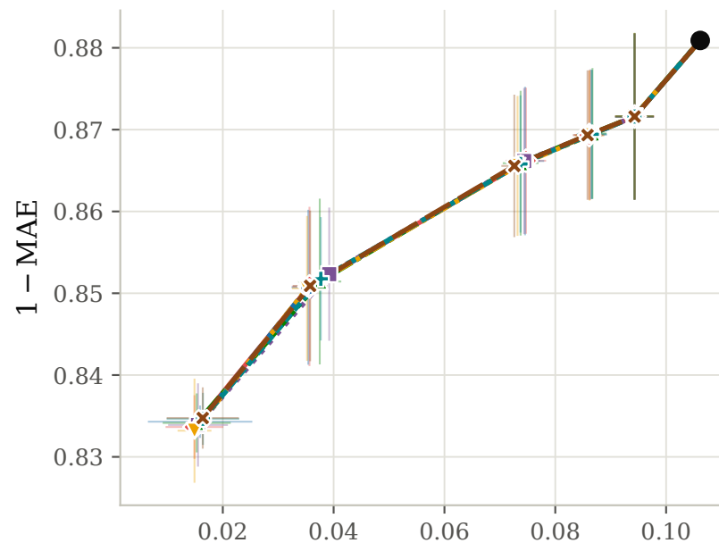
Crime
