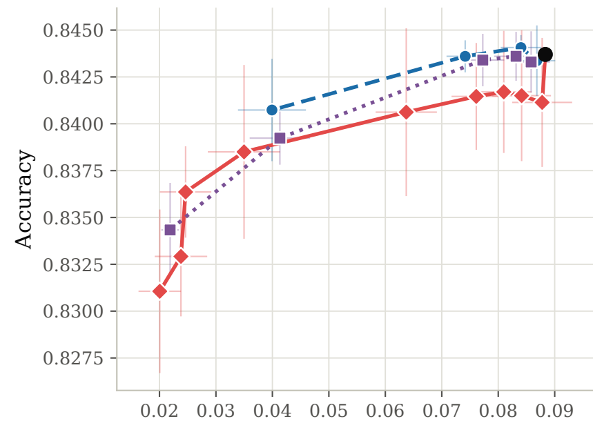
Adult
