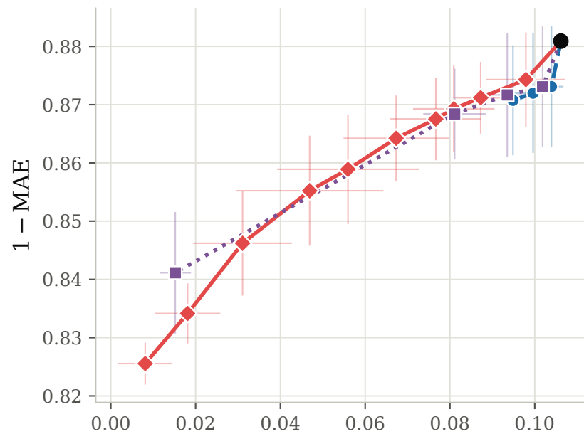
Crime
