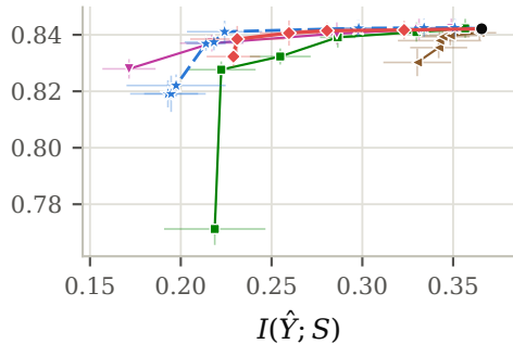
Continuous-S methods
