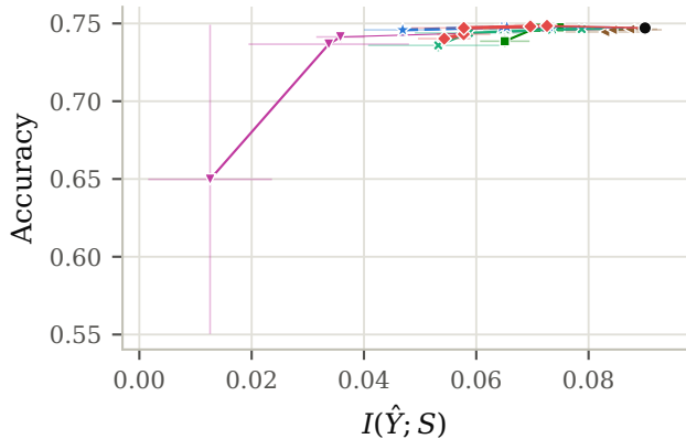
Pokec-z
