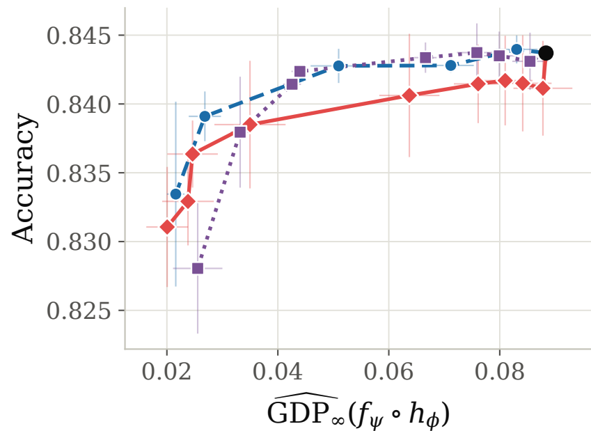
Adult
