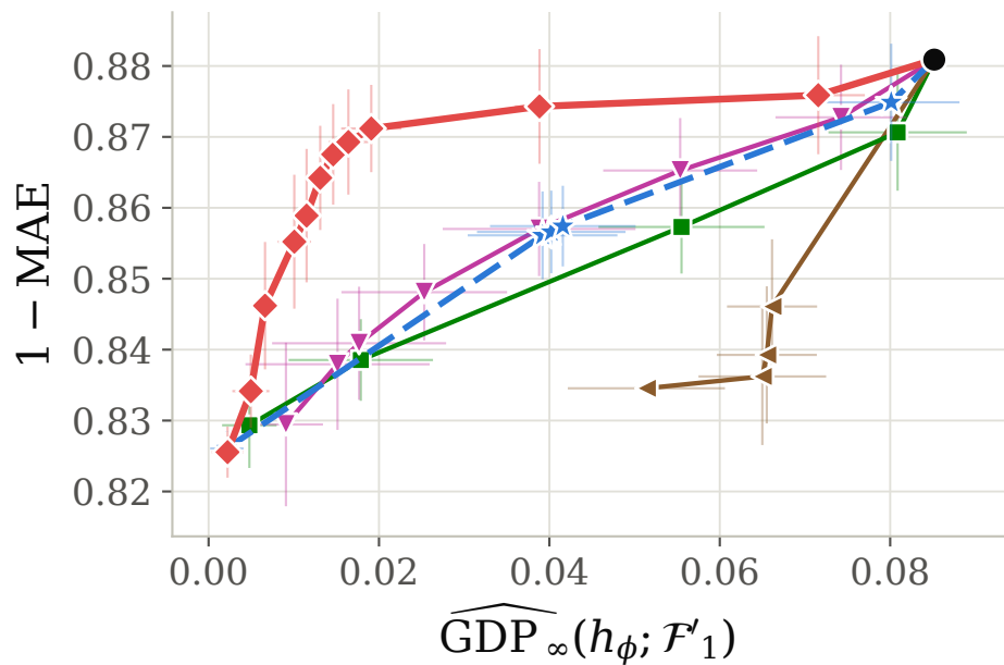
Continuous-S methods
