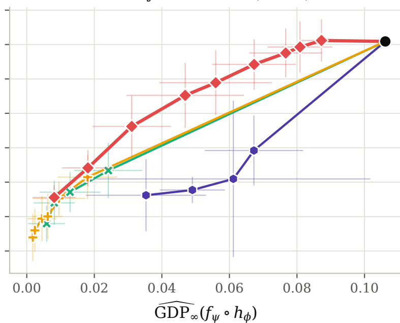
Binary-S methods (mean)
