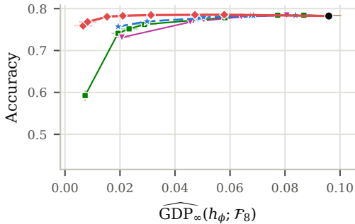
Continuous-S methods
