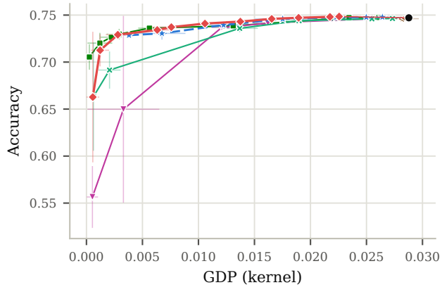
Pokec-z
