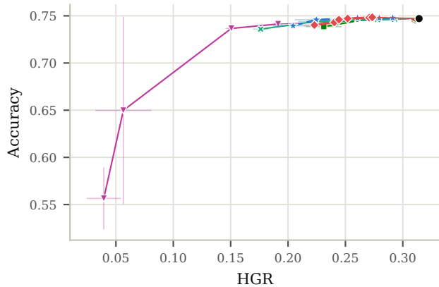
Pokec-z
