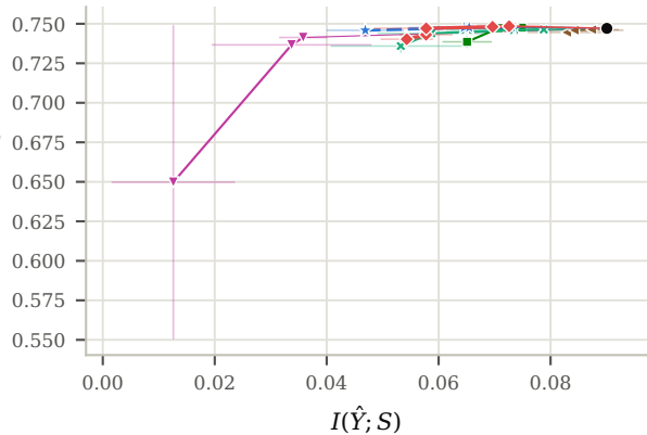
Pokec-z
