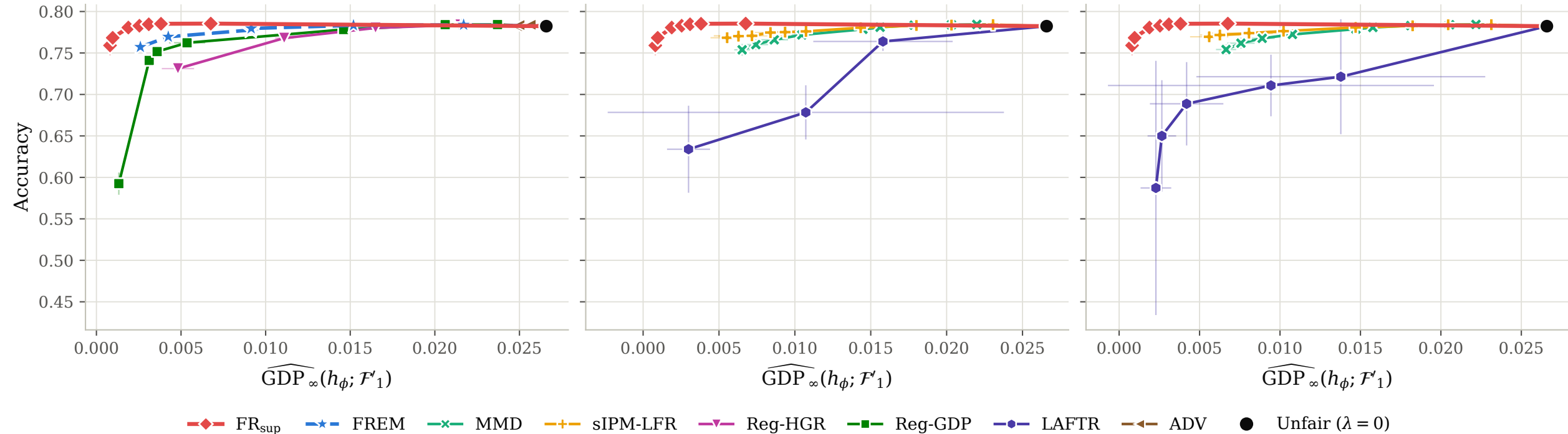
Continuous-S methods
