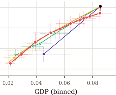
Binary S (median)
