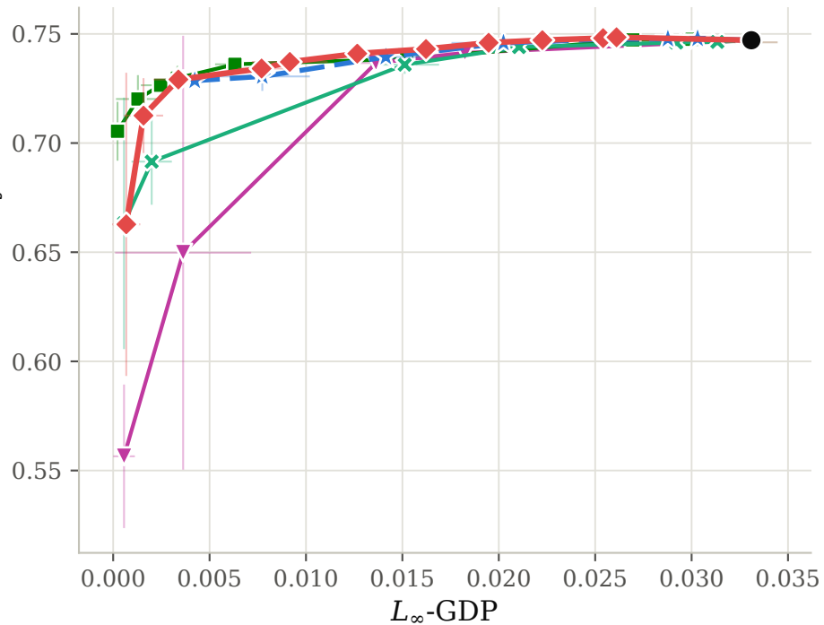
Pokec-z
