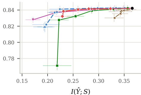
Continuous-S methods
