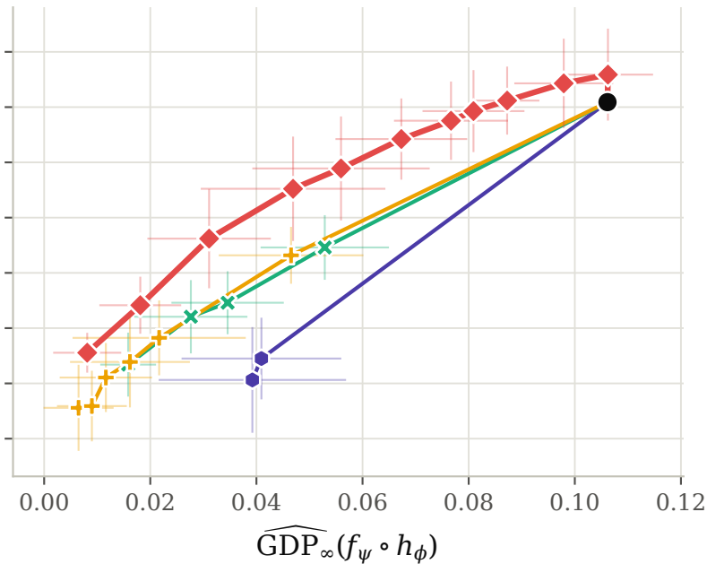
Binary-S methods (median)
