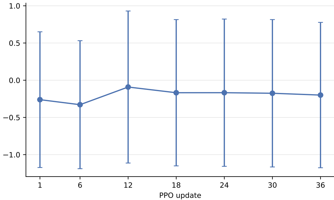
Episode return (mean \pm std)
