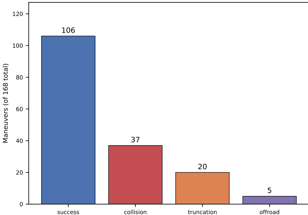
Phase 3 robustness result (168 maneuvers, frenet_mpc, MERGE-every-step) Engineering survivability stimulus -- NOT the final FSM-vs-PPO comparison
