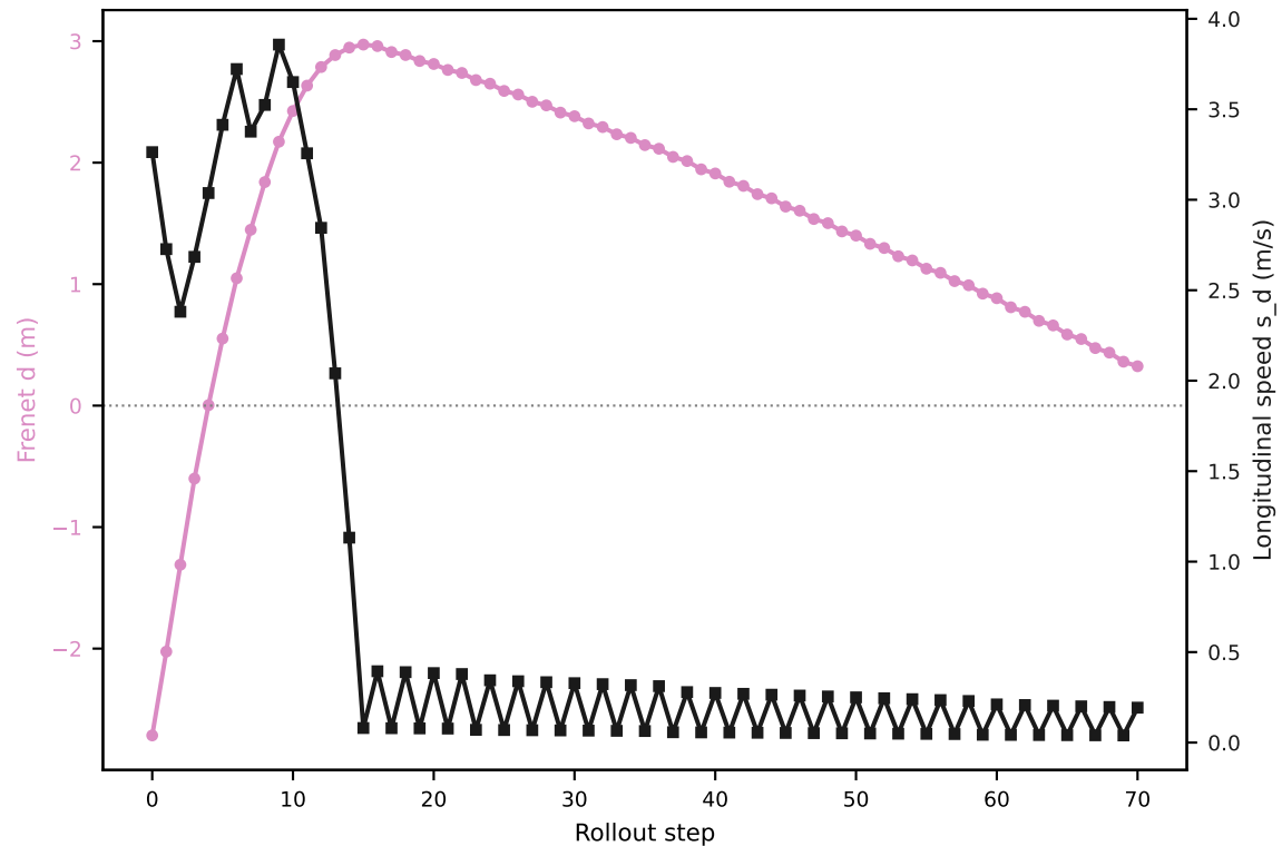
MAN_0107 -- Phase 3 downstream limitation example (NOT FSM/PPO result) Lateral (d) oscillation + longitudinal near-stall in the MERGE target frame; chain never advances, episode truncation_horizon
