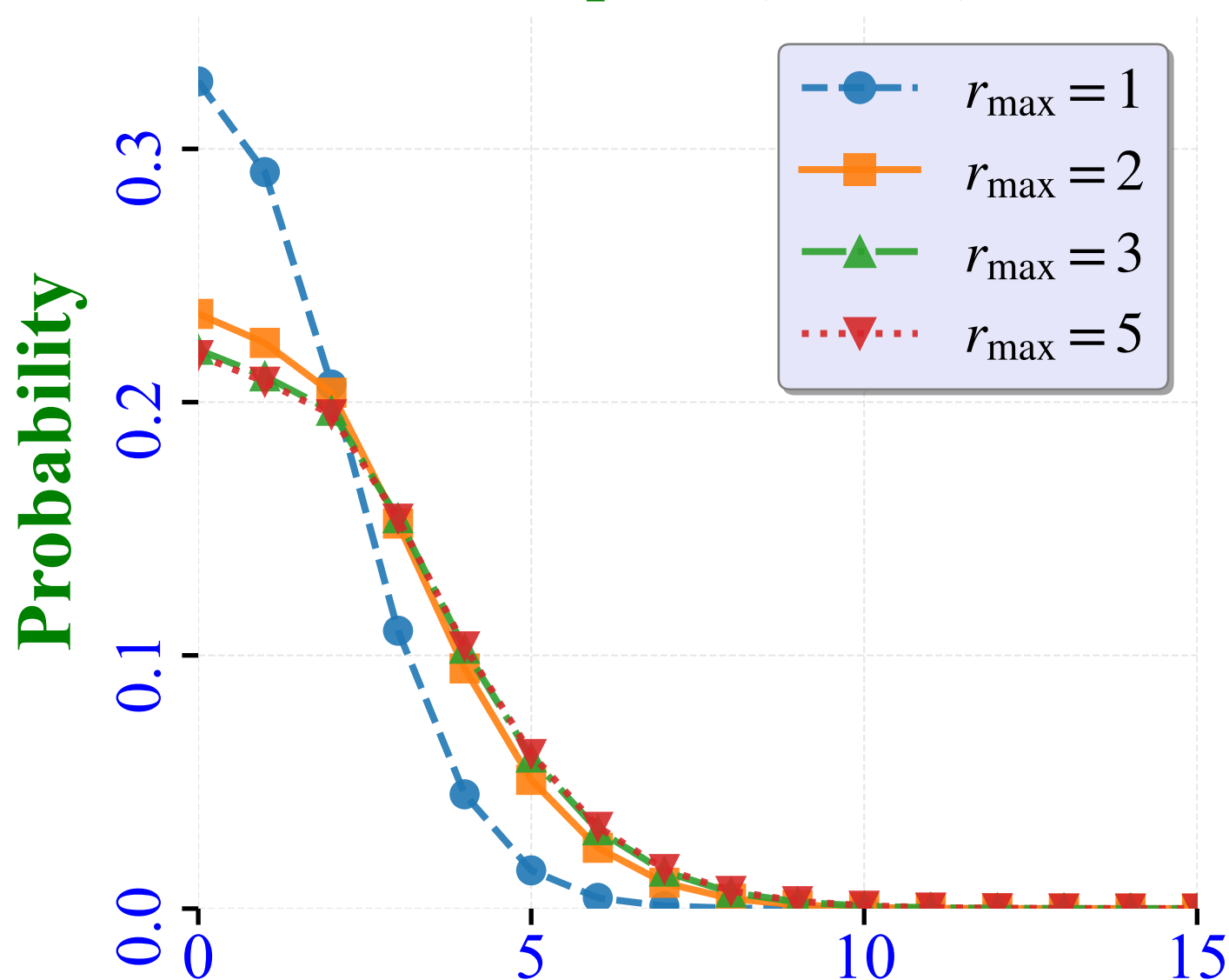
Example 3 ( \alpha = 0.5 )
