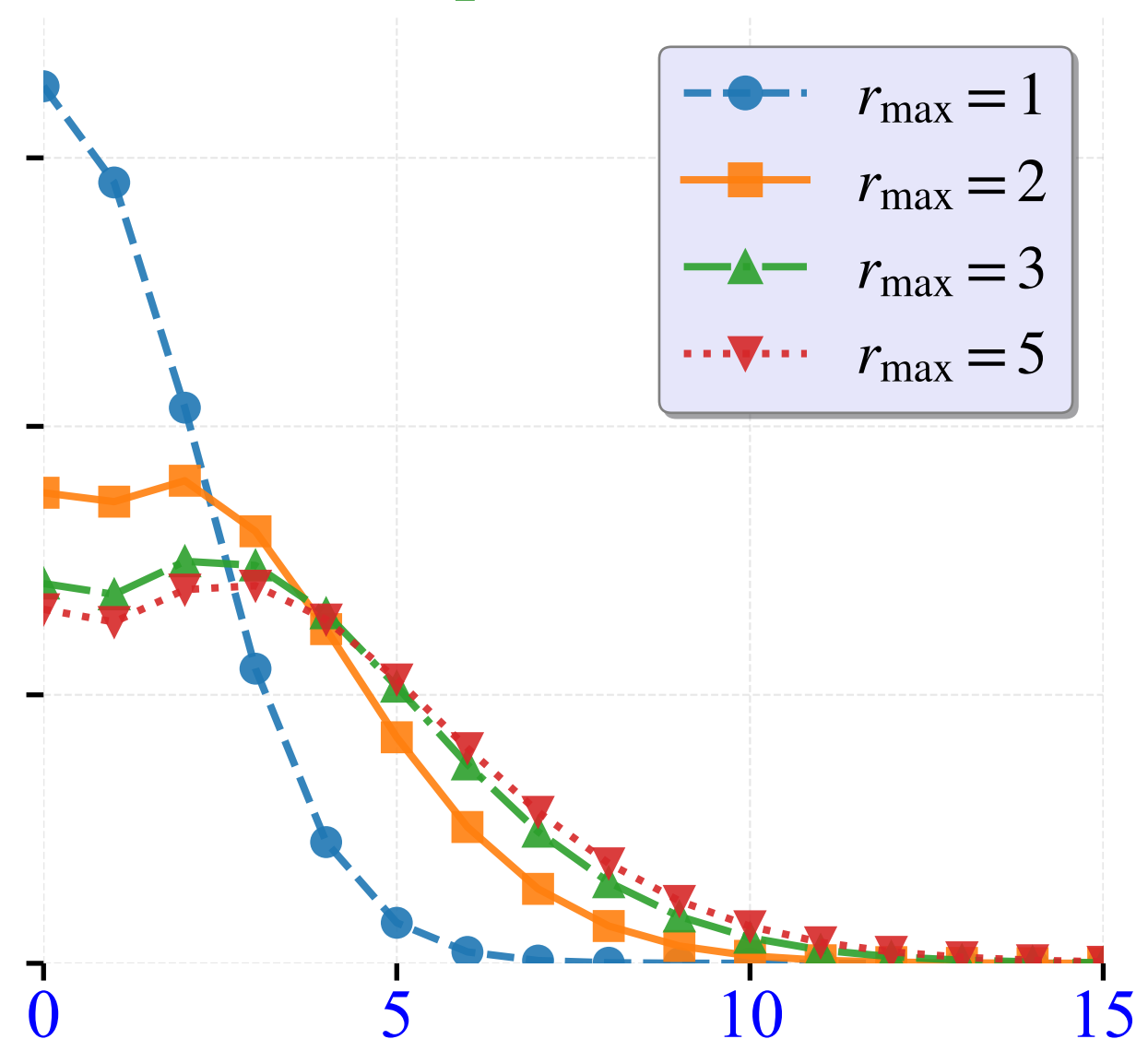
Example 4 ( \alpha = 1.0 )
