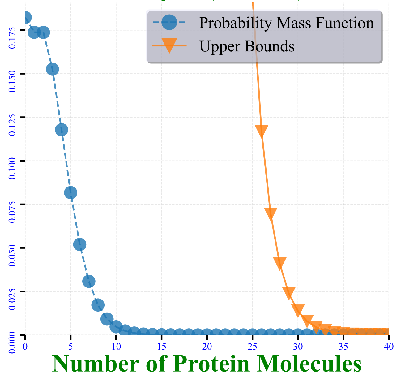
Example 4 ( \lambda = 0.30 )
