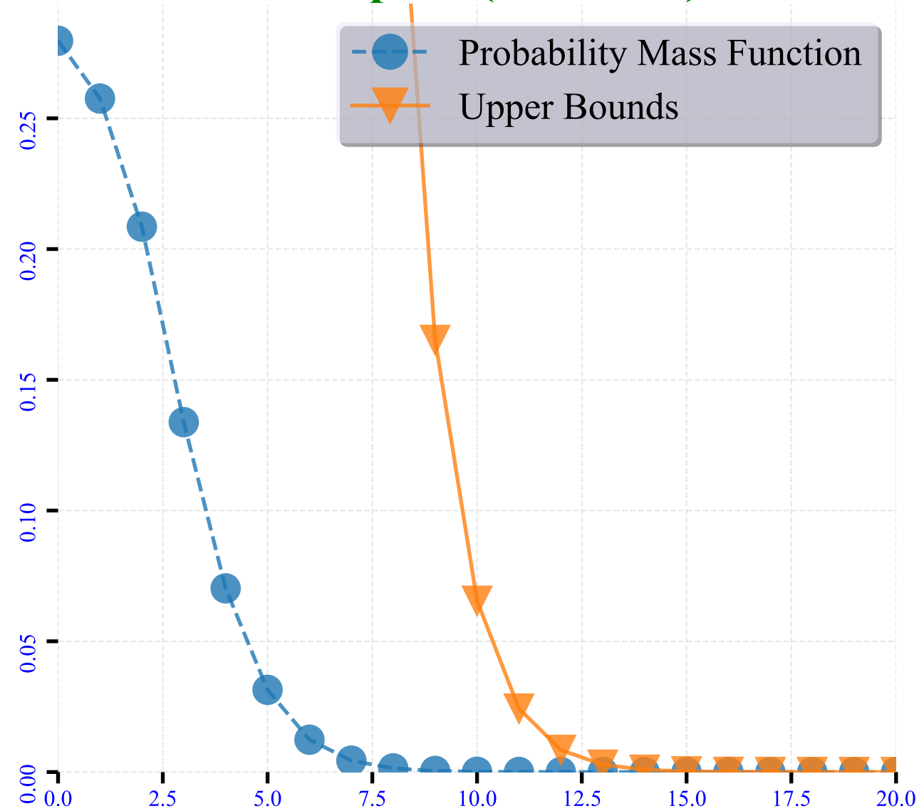
Example 4 ( \lambda = 0.30 )
