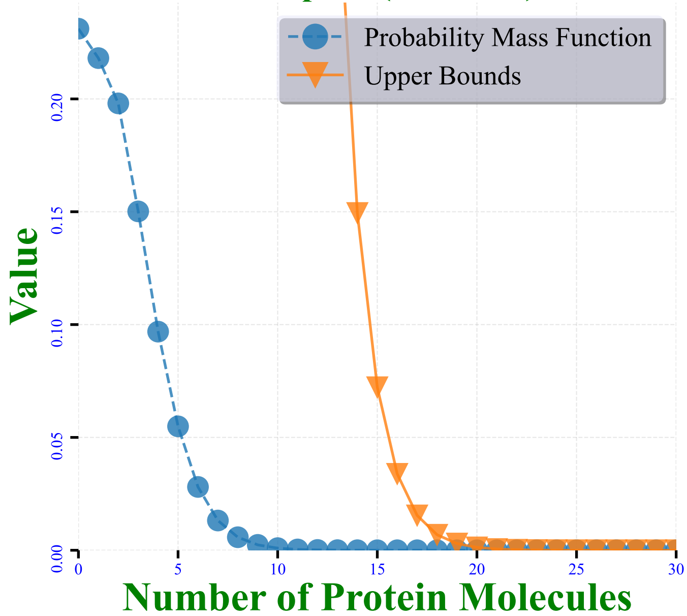
Example 3 ( \lambda = 0.20 )
