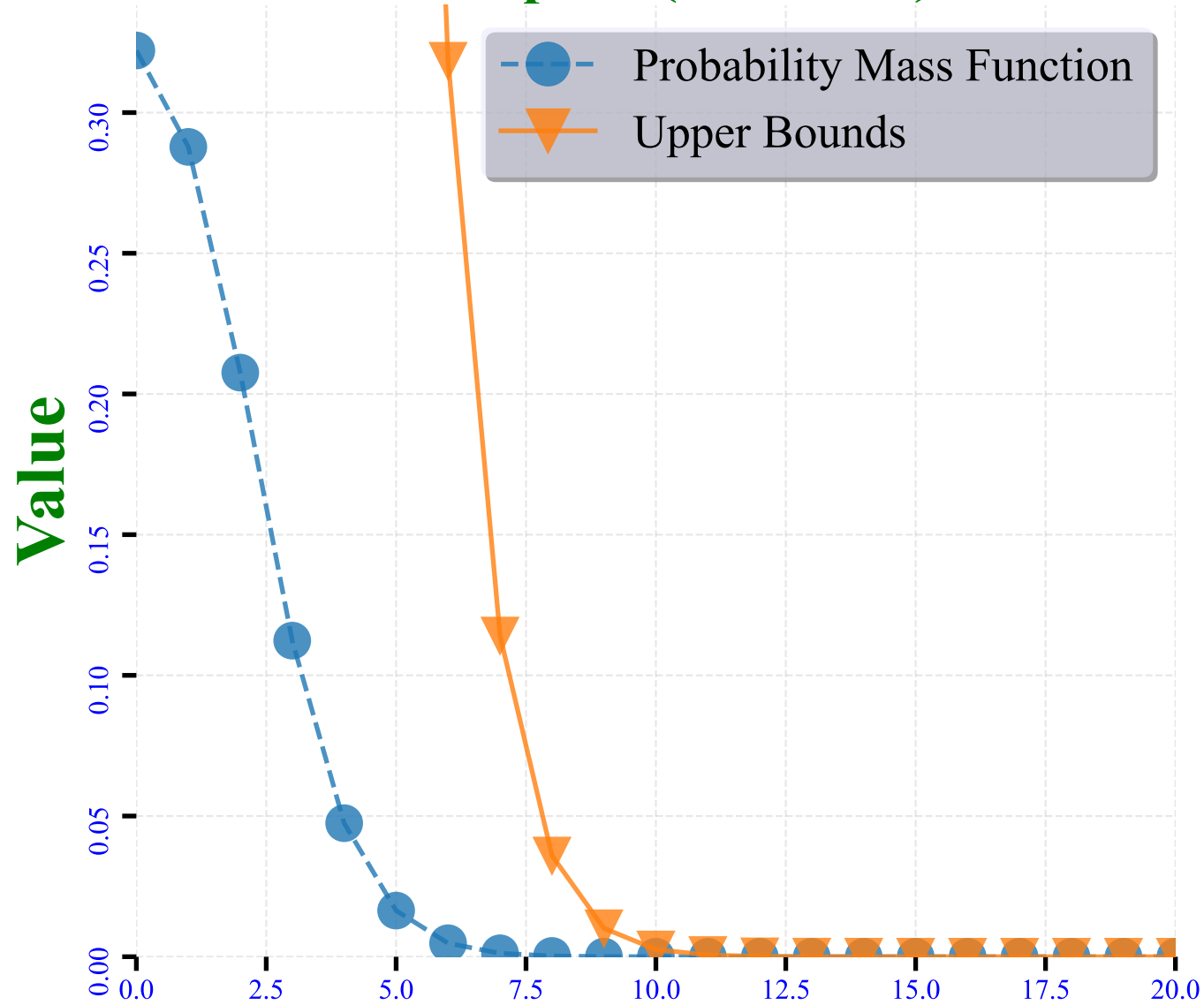
Example 3 ( \lambda = 0.20 )
