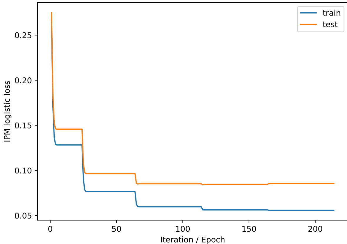
IPM logistic loss
