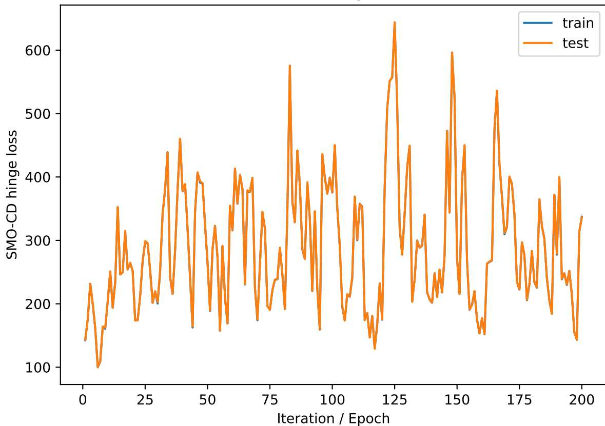
SMO-CD hinge loss
