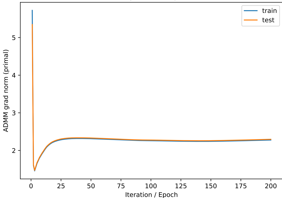
ADMM grad norm (primal)
