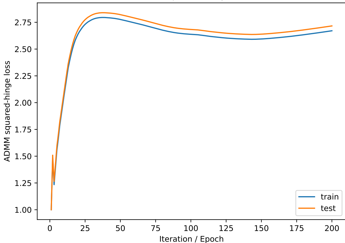
ADMM squared-hinge loss
