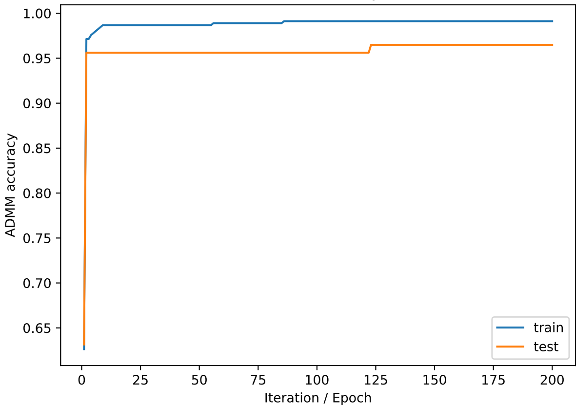
ADMM accuracy
