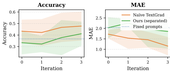
Figure 4: Synthetic underwriting: accuracy and MAE vs. optimization iteration (mean \pm std over 3 seeds). Our method (green) maintains 100% stability throughout.
