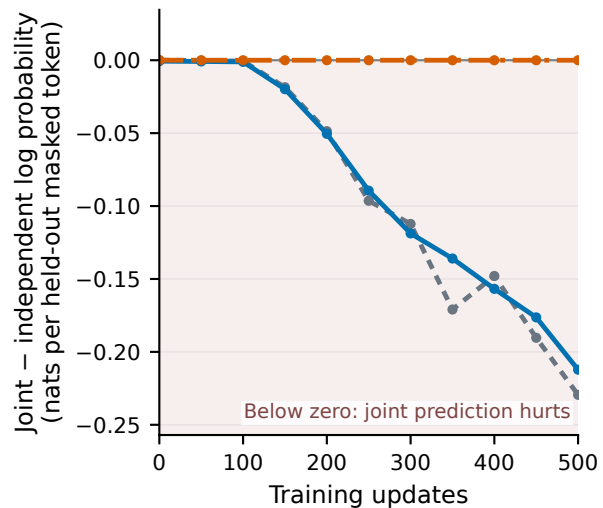
Do token relationships help?
