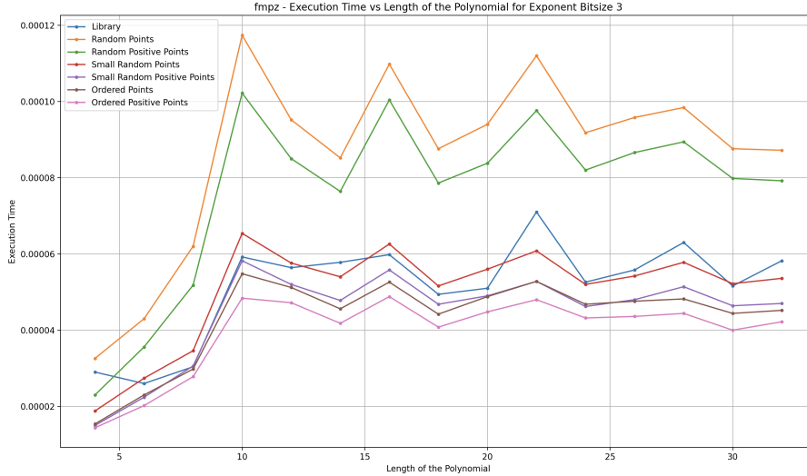
Figure 1: FMPZ bivariate polynomial resultant execution time (in seconds) for exponent bit size 3 with varying lengths.
