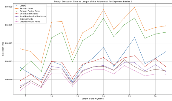
(a) FMPQ bivariate polynomial resultant execution time (in seconds) for exponent bitsize 3 with varying lengths.
